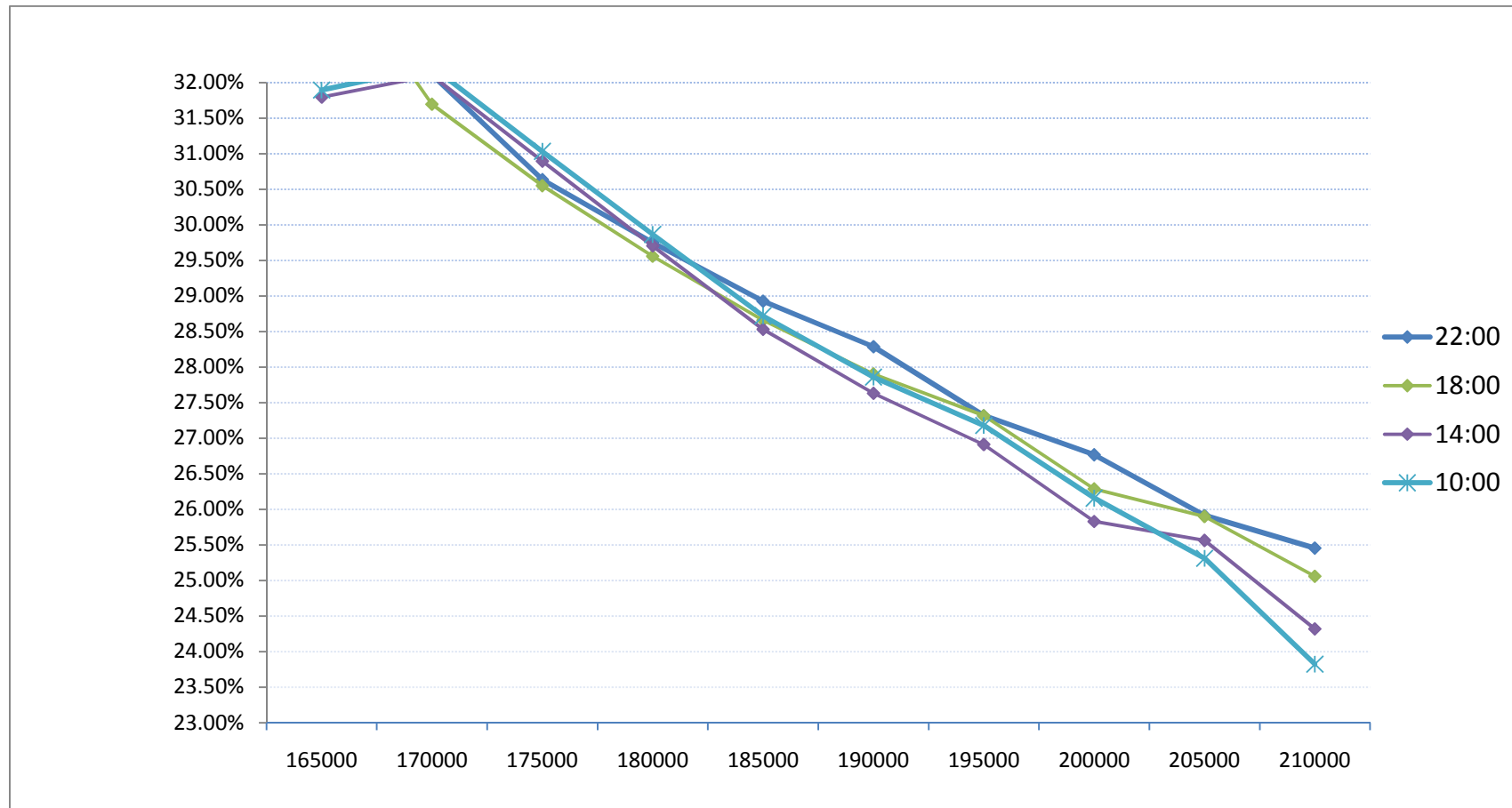
RTS intraday volatility curve (as of 05-04-11)
